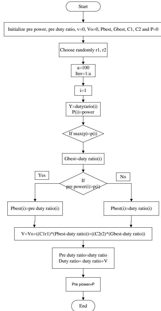
Figure 5: MPPT Procedure Utilizing Particle Swarm Optimization Technique
