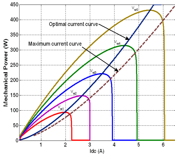
Figure 2: Characteristics of Turbine Power as a Function of the DC Side Current
